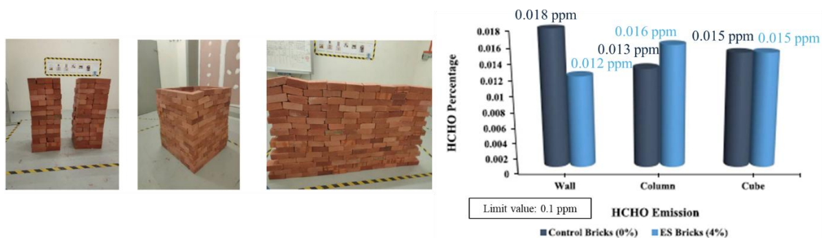
Figure 5. Clay bricks made of ES in the form of column, cube and wall (left), HCHO emissions of control sample and samples with ES (Abdul Kadir et al. 2023)
