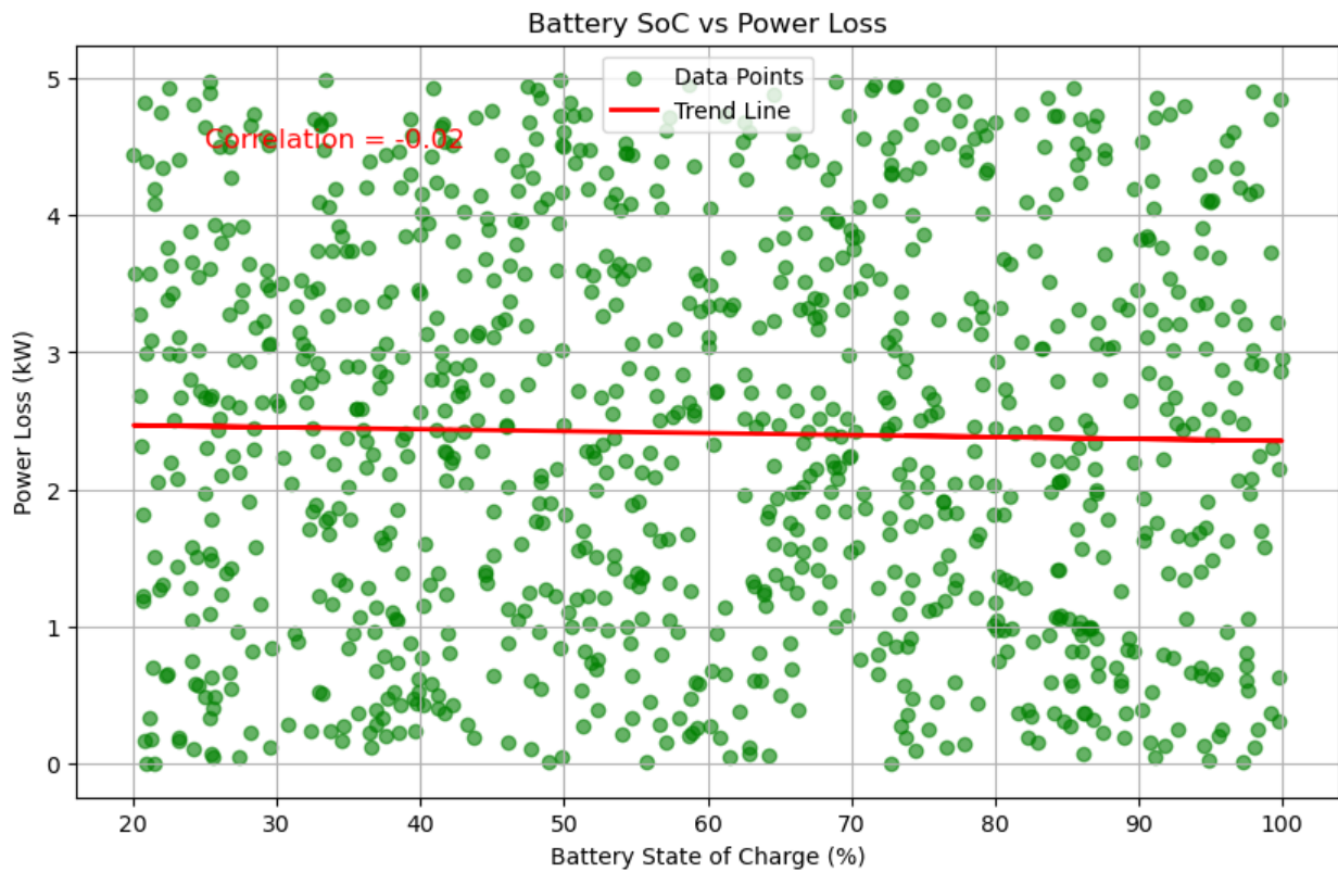
Figure 4.11: Battery SoC vs Power Loss
