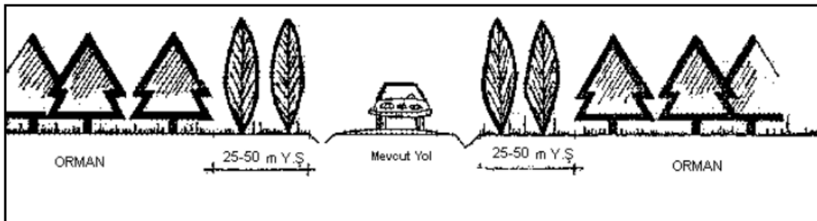
Figure 11. Double-sided fire safety strip
