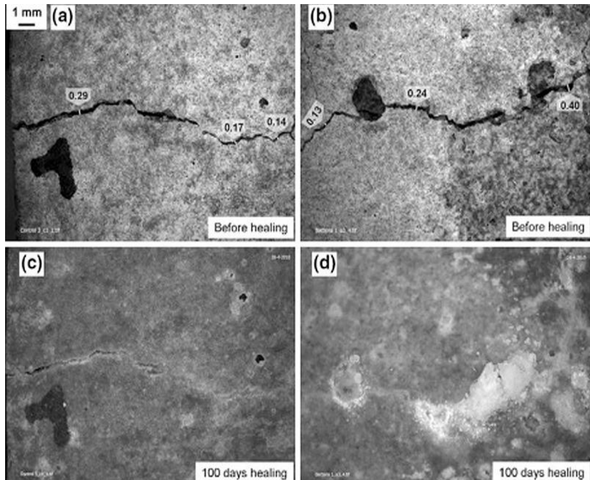
Figure 1 How self-healing concrete works.[1]
