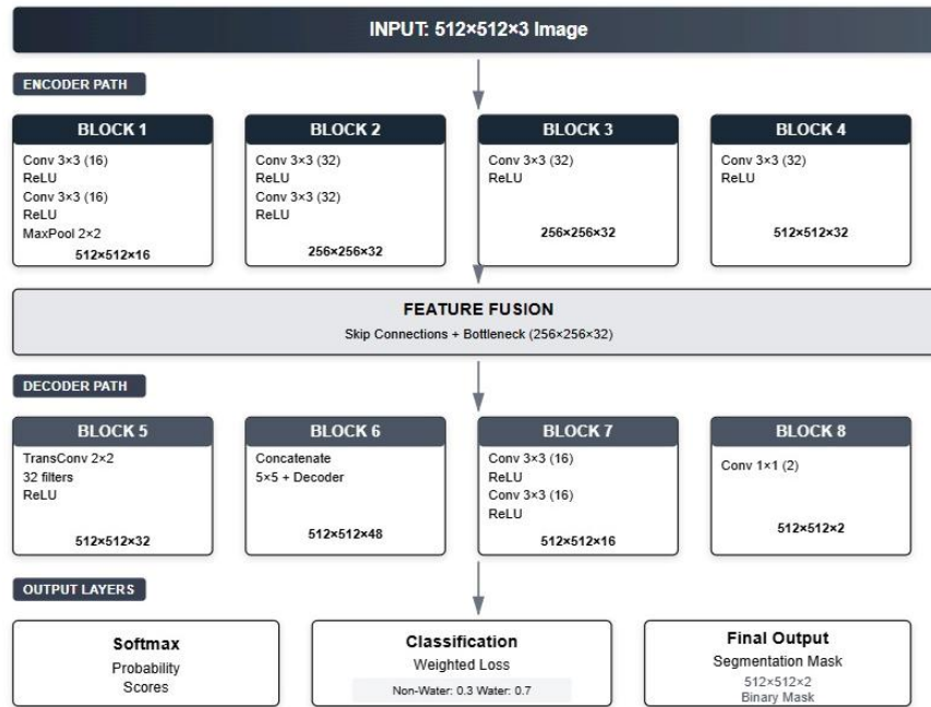
Figure 1. ERCNet Network Architecture
