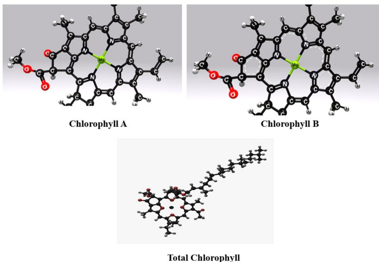
Figure 1. The molecular structure of chlorophyll (Anonymous, 2025)
