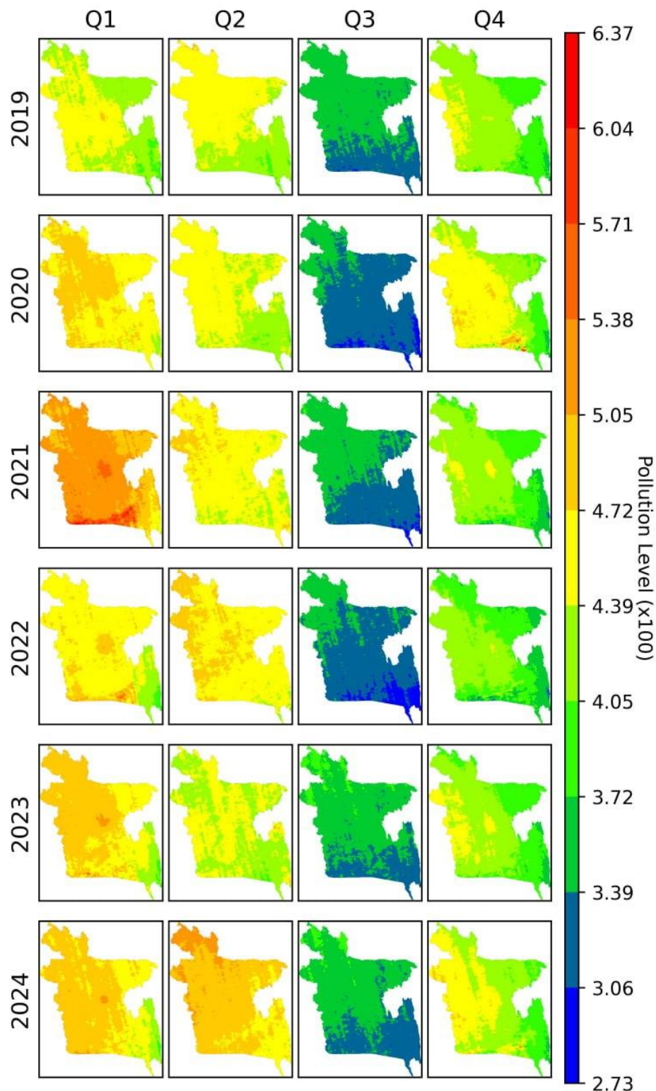
Figure 3:10 Seasonal CO variation mapping from 2019 to 2024 in Bangladesh
