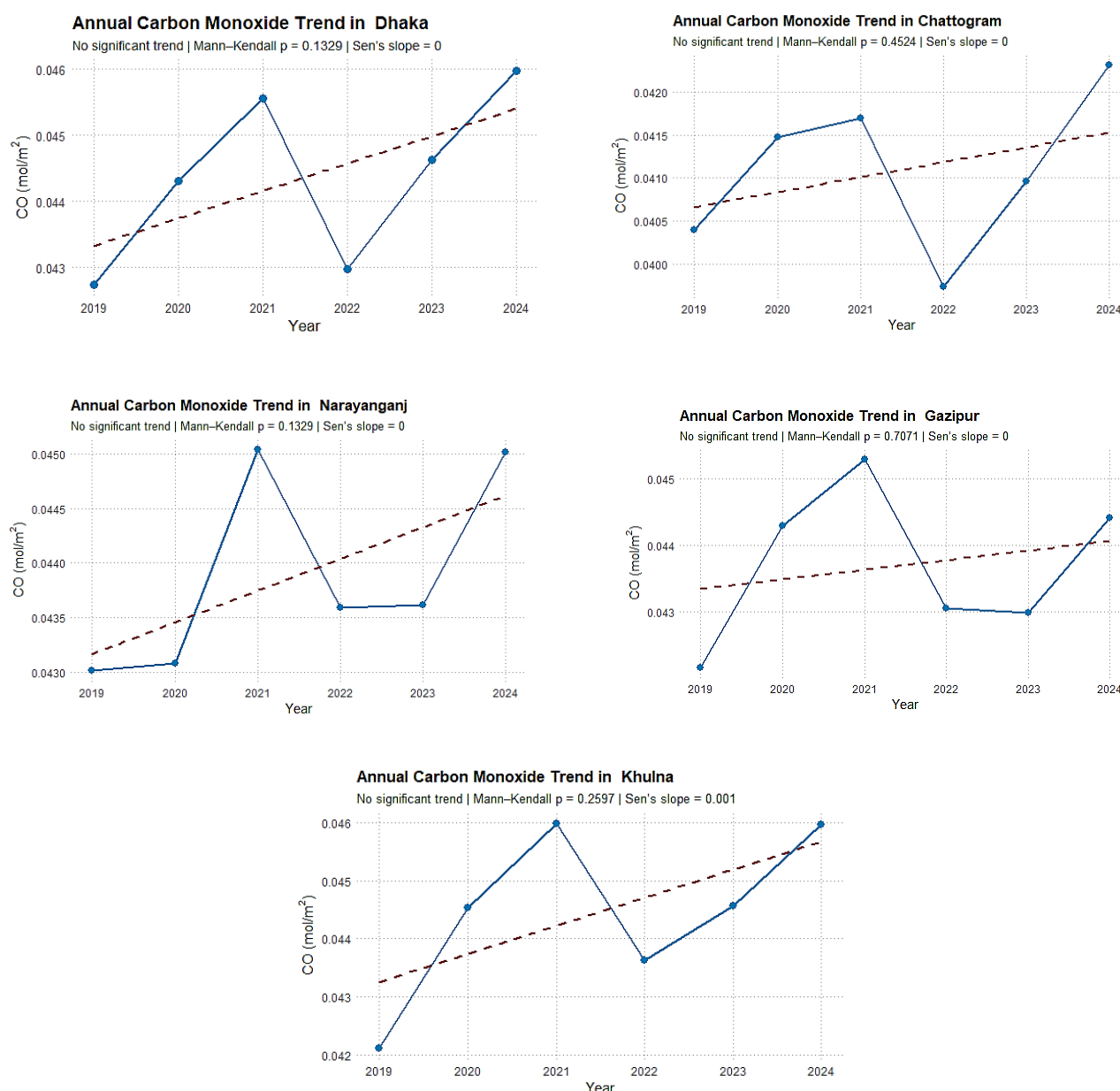
Figure 3:11 Mann-Kendall and Sen's slope test of maximum CO concentration (2019–2024) in five industrial cities of Bangladesh
