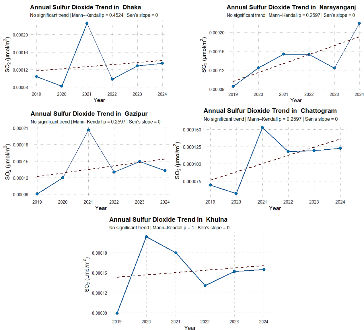
Figure 3:5 Mann-Kendall and Sen's slope test of maximum \text{SO}_2 concentration (2019–2024) in five industrial cities of Bangladesh
