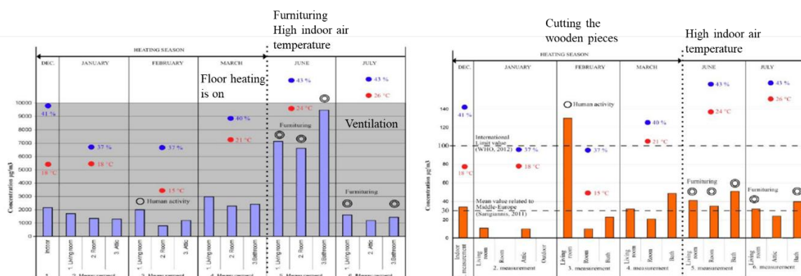
Figure 4. TVOC (left) and HCHO (right) results of the passive, wooden-framed house (red dots represent indoor temperature and blue demonstrates indoor relative humidity (Patko et al. 2024))
