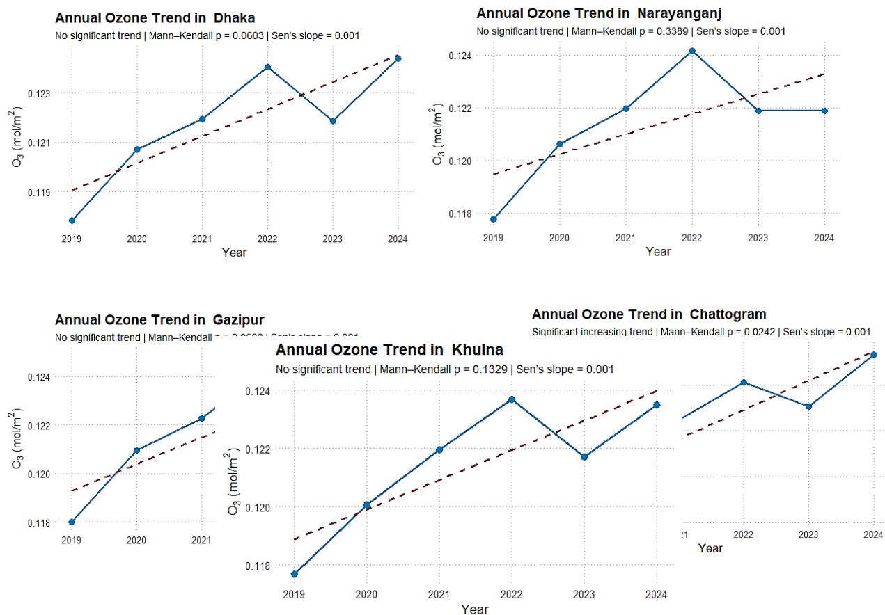
Figure 3:8 Mann–Kendall and Sen’s slope test of maximum O_3 concentration (2019–2024) in five industrial cities of Bangladesh
