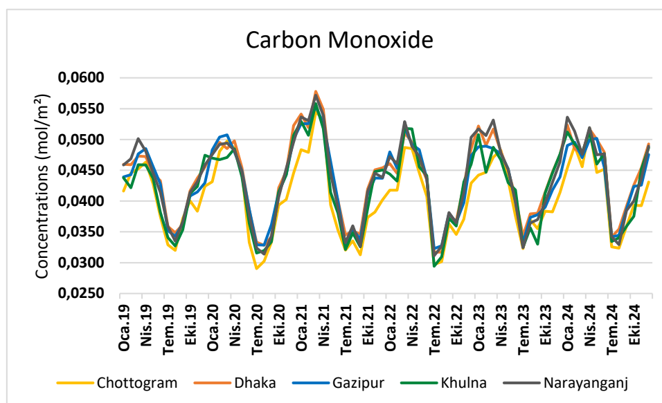
Figure 3:12 Temporal trends of CO from 2019 to 2024 in major cities of Bangladesh
