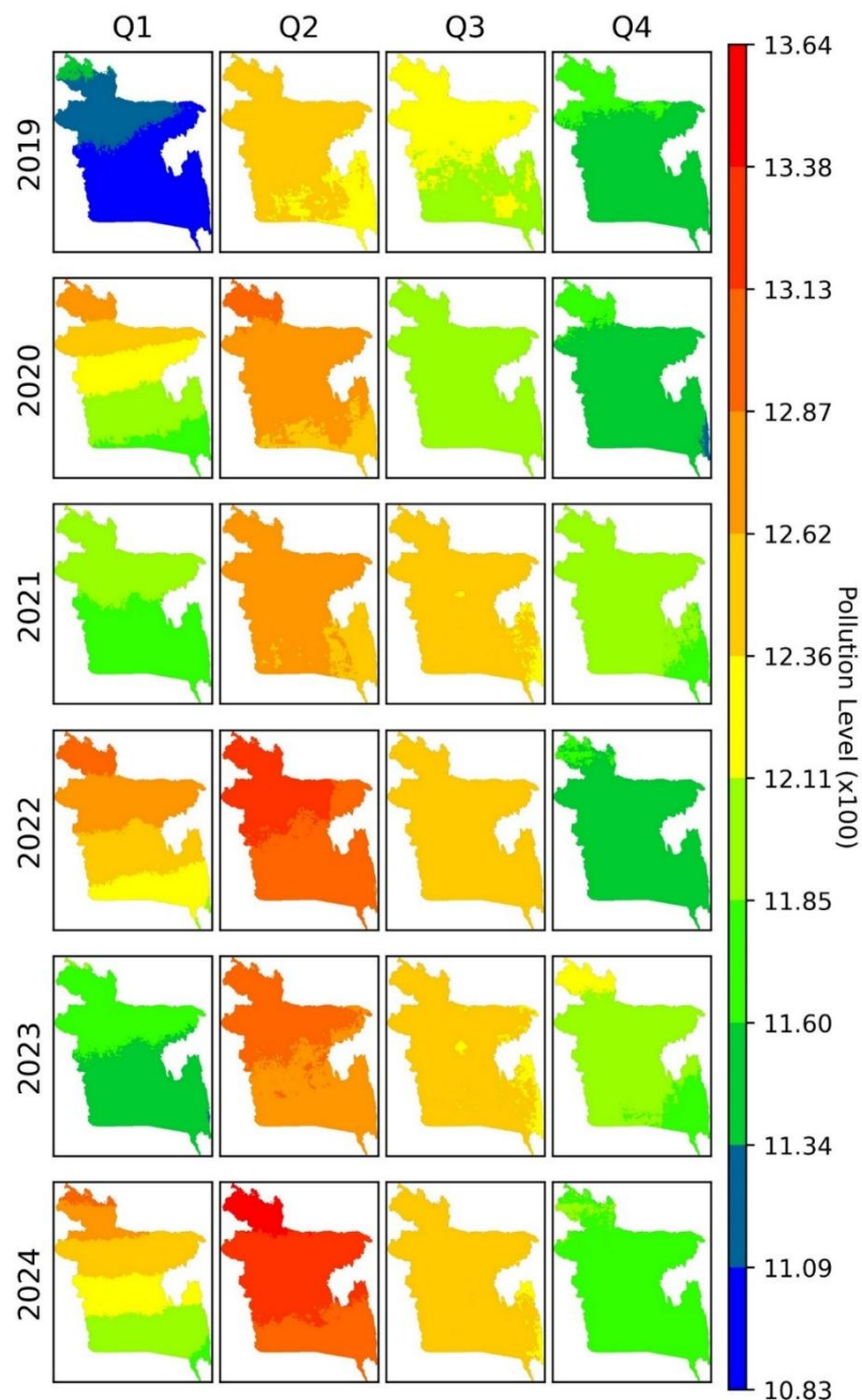
Figure 3:7 Seasonal \text{O}_3 variation mapping from 2019 to 2024 in Bangladesh
