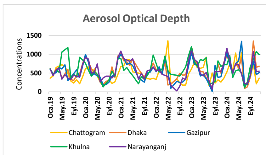
Temporal trends of AOD from 2019 to 2024 in major cities of Bangladesh
