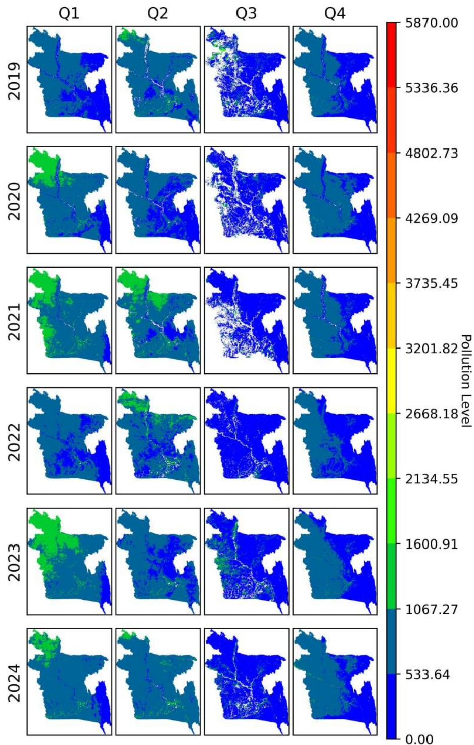
Figure 3:13 Seasonal AOD variation mapping from 2019 to 2024 in Bangladesh
