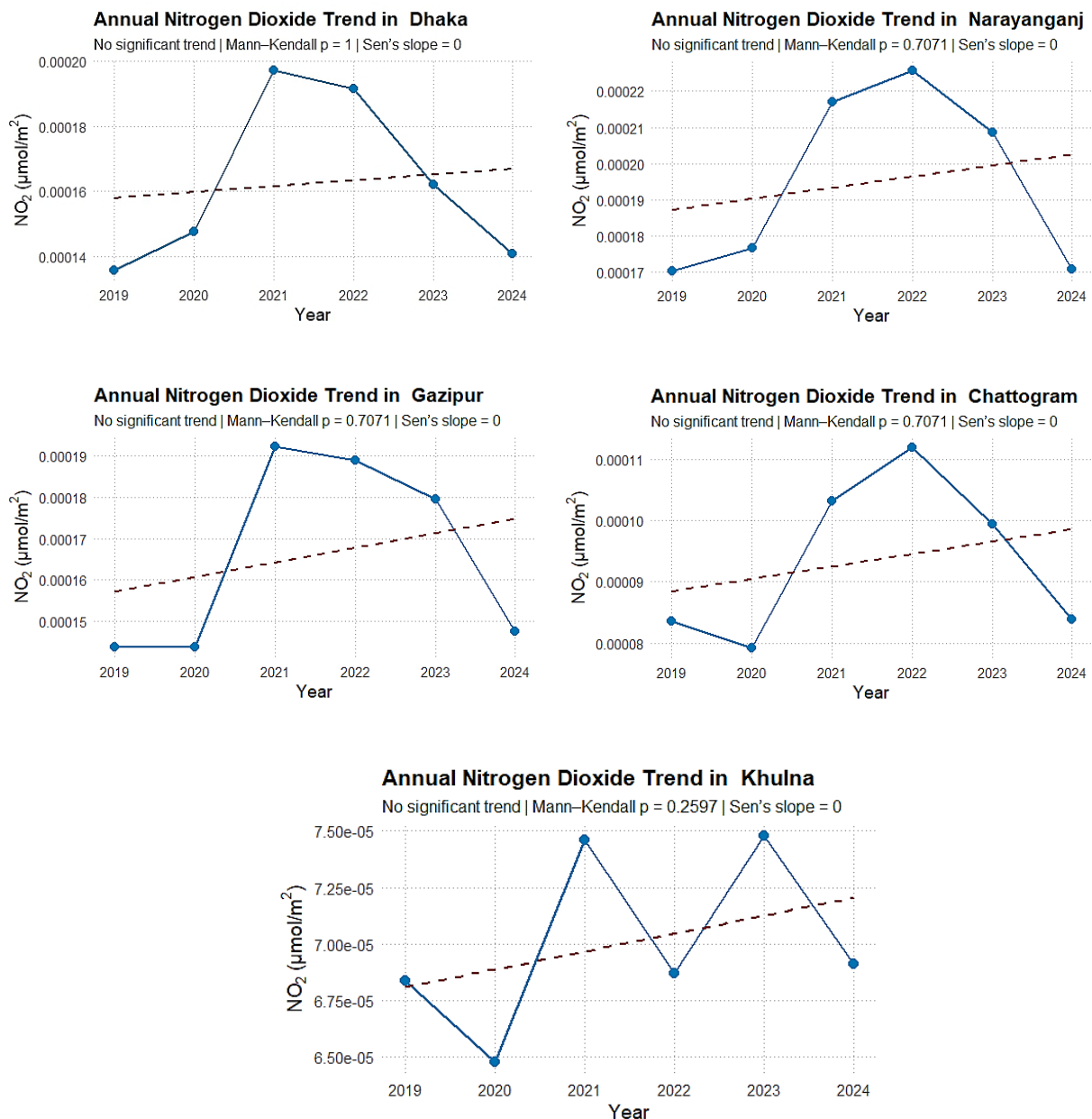
Figure 3:2 Mann-Kendall test of maximum \text{NO}_2 concentration (2019–2024) in five industrial cities
