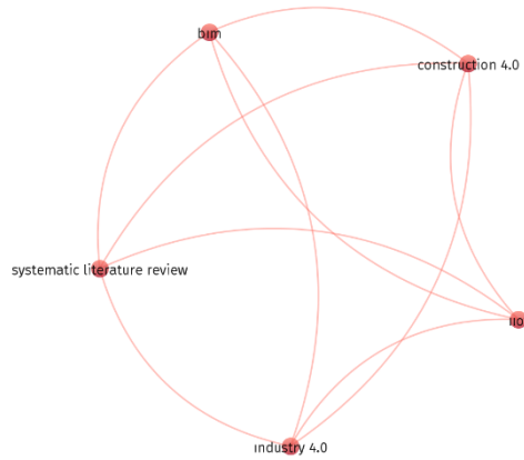
Figure 8. Keyword Map
