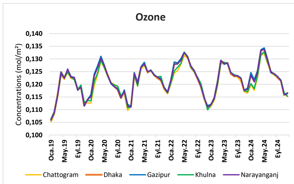
Figure 3:9 Temporal trends of O_3 from 2019 to 2024 in major cities of Bangladesh
