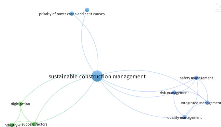
Figure 7. Keyword Map
