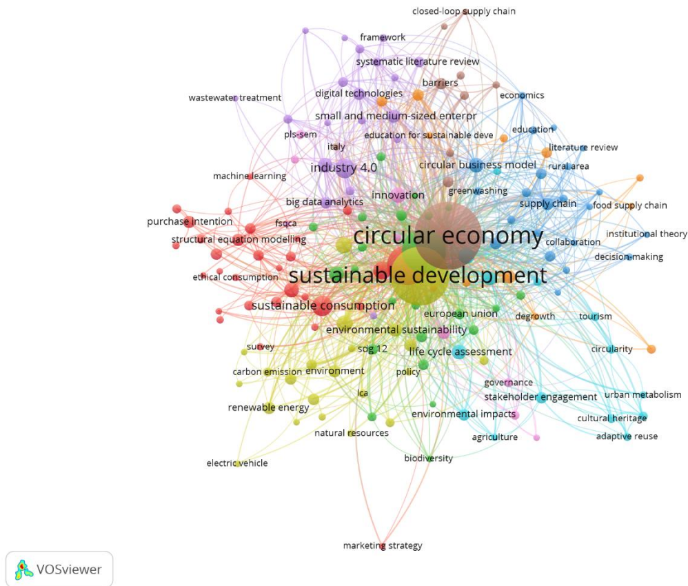
Figure 5. Co-occurrence Analysis
