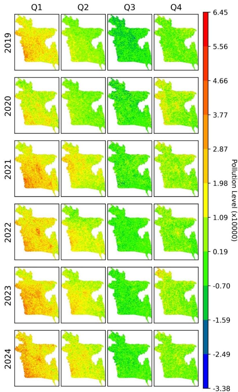
Figure 3:4 Seasonal SO 2 variation mapping from 2019 to 2024 in Bangladesh
