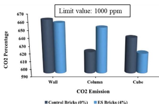
Fig. 5. Carbon dioxide emissions from different types of fired clay bricks.
