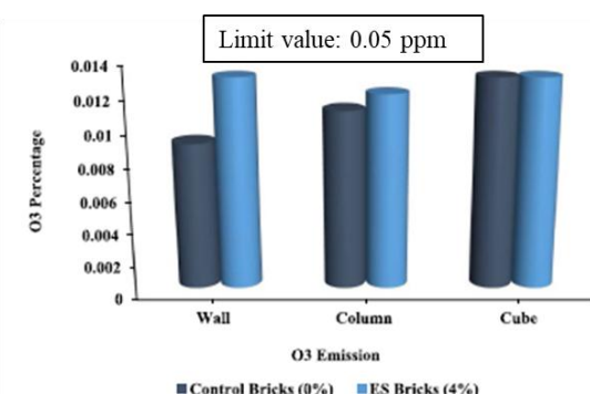
Figure 6. Ozone and Particulate matter (PM10) emissions of control sample and samples with electroplating sludge (ES) (Abdul Kadir et al. 2023)
