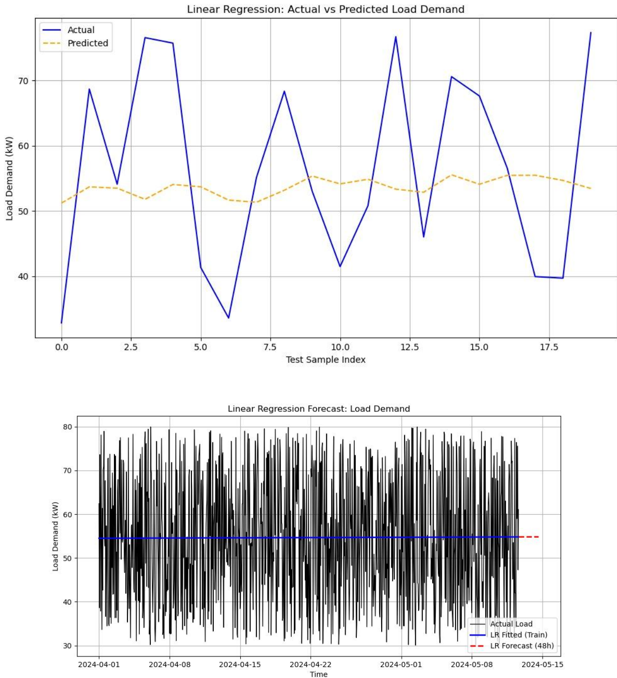
Figure 4.5: Linear Regression – Actual vs Predicted Load Demand
