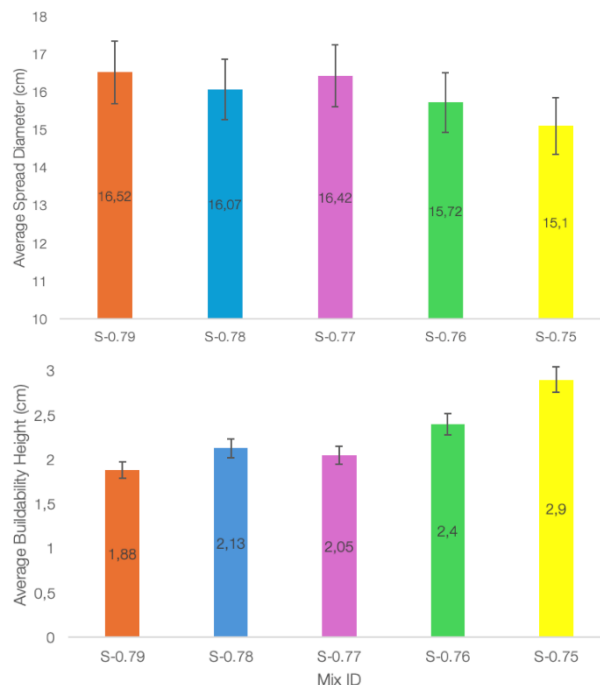
Figure 3. Comparison of fresh-state properties for slag-based geopolymer mixtures with varying activator-to-binder ratios. (Top) Average spread diameter from flow table tests; (Bottom) average retained height under 600 g load indicating buildability performance.
