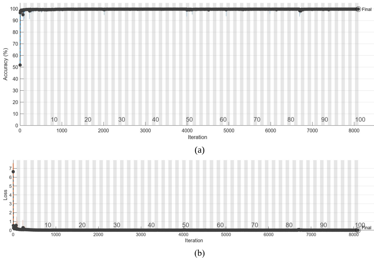
Figure 2. Change in Accuracy (a) and Loss (b) values of the ERCNet model during the training process concerning iterations.
