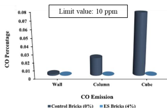
Fig. 6. Carbon monoxide (CO) emissions from different types of fired clay bricks.
