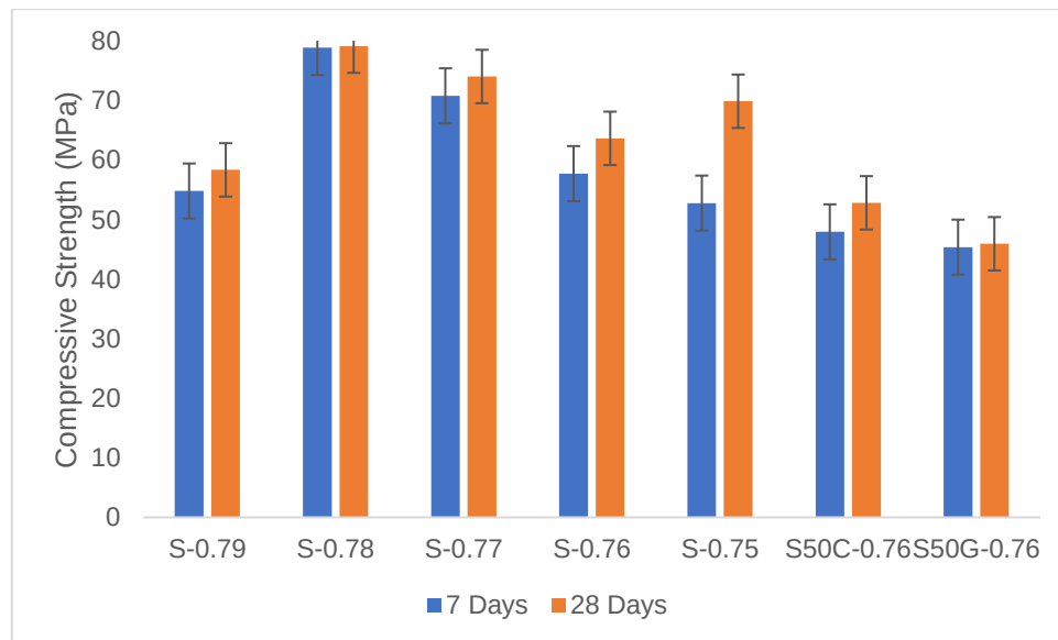
Figure 5. Evolution of compressive strength at 7 and 28 days for slag-based reference mixes and modified mixes incorporating ceramic (S50C-0.76) and glass powder (S50G-0.76).
