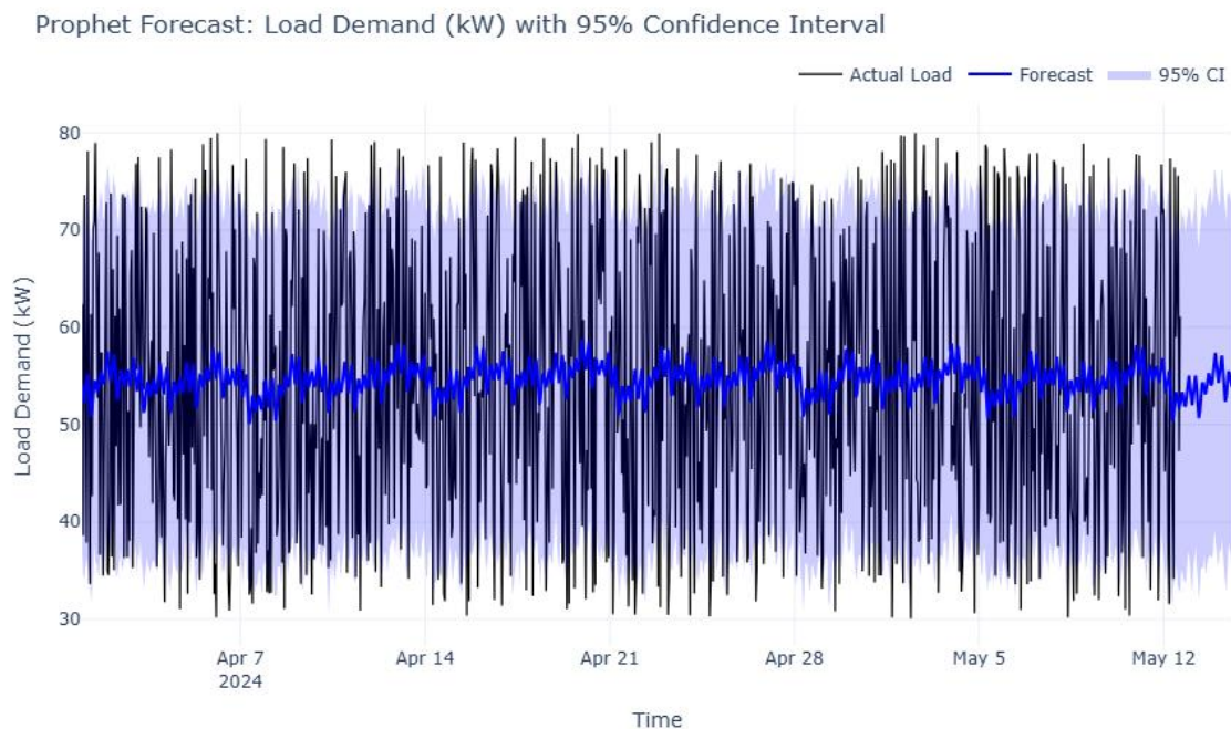
Figure 4.4: Prophet Model – Daily Average Forecast (95% CI)
