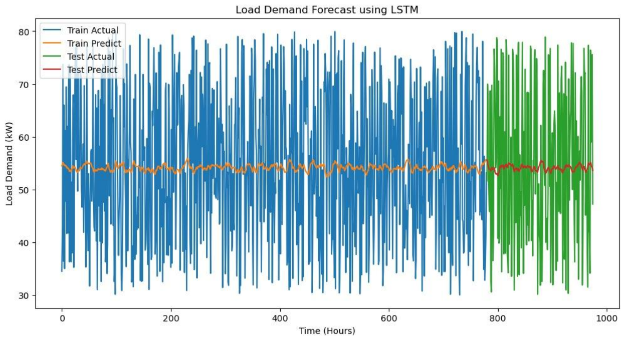
Figure 4.3: LSTM Model – Train Actual, Train Predict, Test Actual, Test Predict
