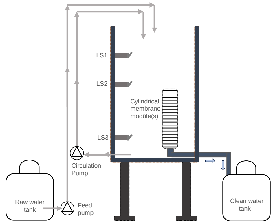
Figure 1. Schematic diagram of the GD-DM reactor
