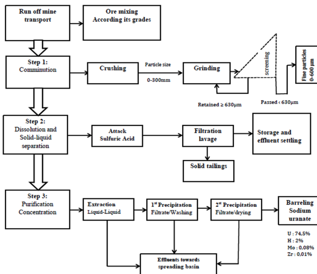
Figure 2. Flowsheet of uranium ore processing.
