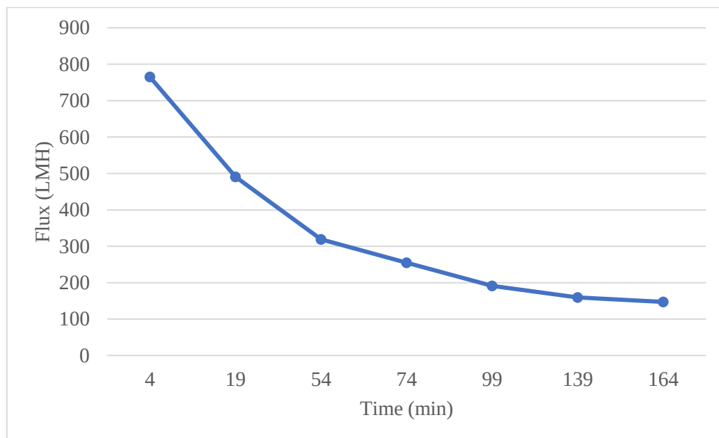
Figure 1. Flux profile of the reactor operation.
