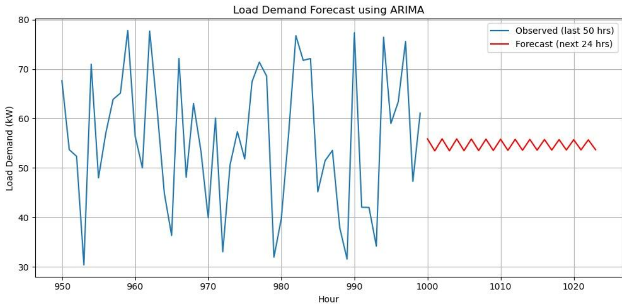
Figure 4.2: Load Demand Forecast using ARIMA.
