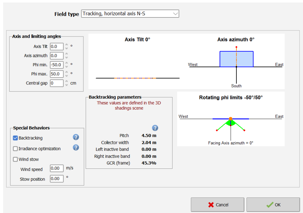
Figure 4. PVsyst orientation interface (tracker orientation and backtracking settings)
