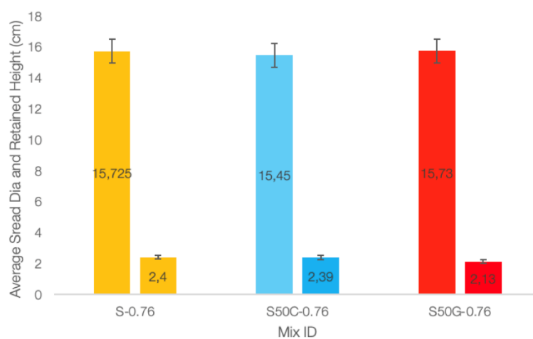
Figure 4. Average spread diameter and retained height for the reference (S-0.76), 50 % ceramic (S50C-0.76), and 50 % glass (S50G-0.76) mixes.
