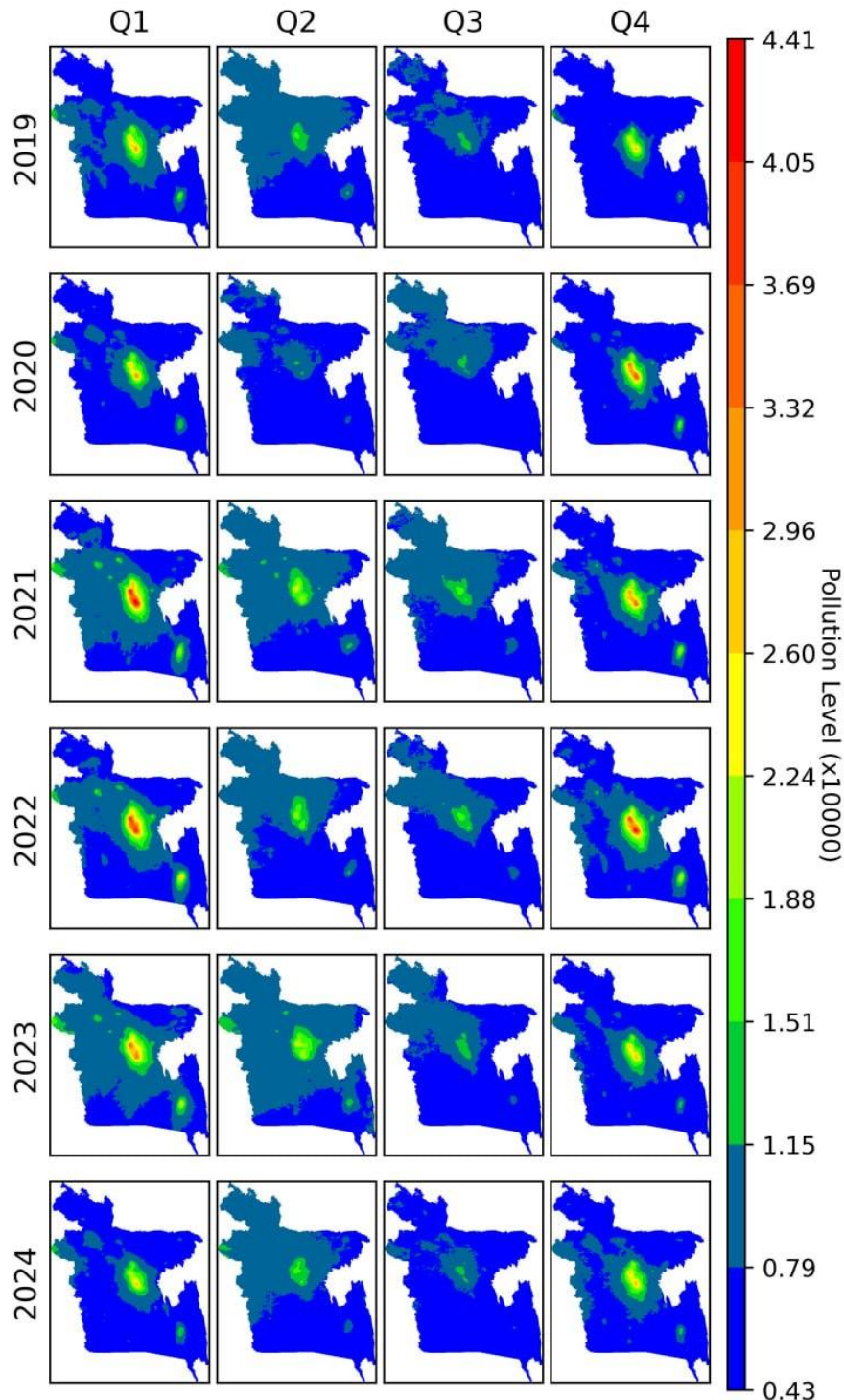
Figure 3:1 Seasonal NO 2 variation mapping from 2019 to 2024 in Bangladesh
