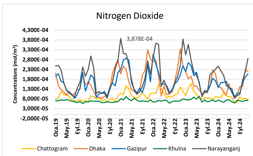
Figure 3:3 Temporal trends of NO 2 from 2019 to 2024 at major cities of Bangladesh
