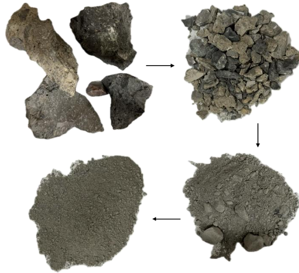
Figure 1. RCA preparation process conducted in our laboratory: collected waste concrete was subjected to jaw crushing, followed by milling in a Los Angeles drum, and subsequently sieved (<2 mm) to obtain fine recycled aggregates for use in geopolymer mixes.
